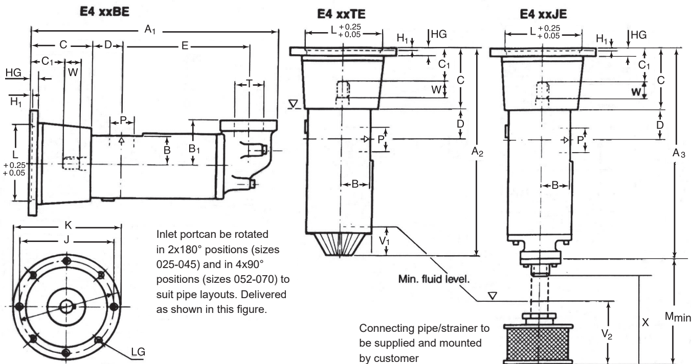
Inlet dimensions (mm)
