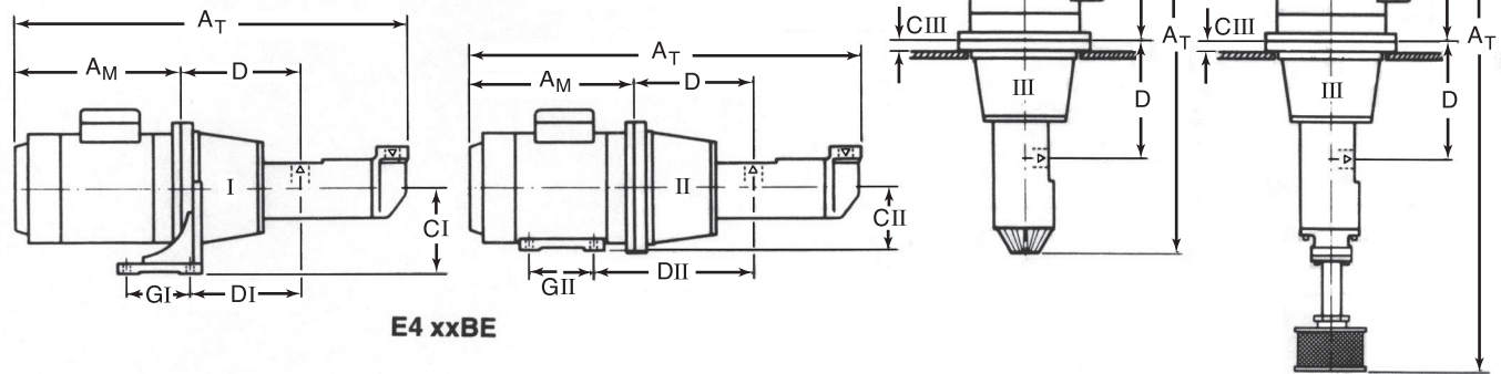
Pump Unit
