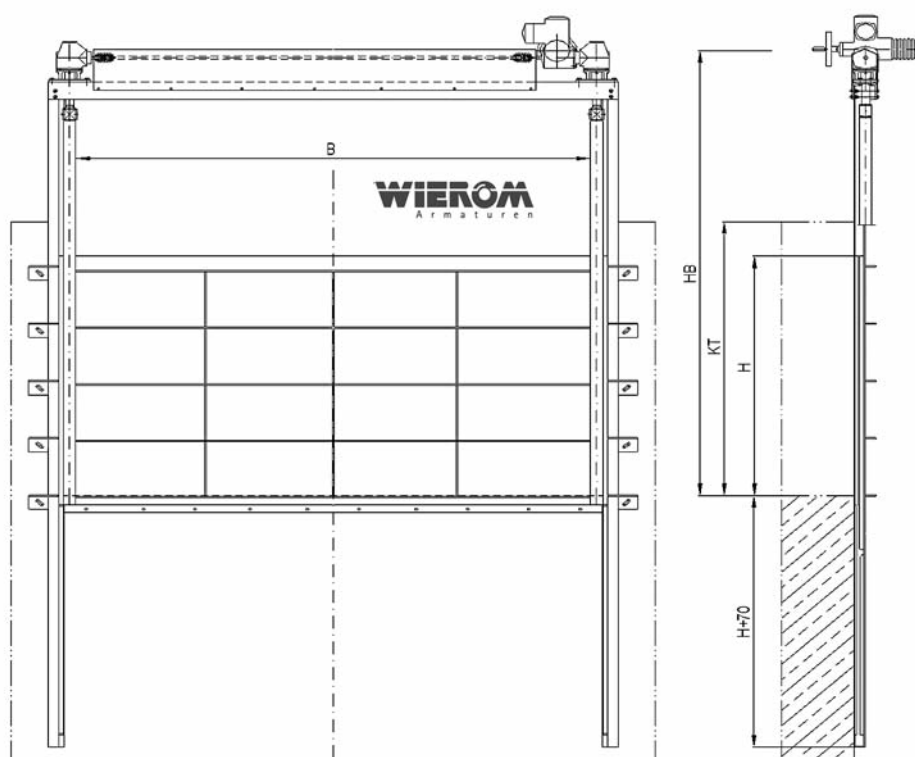
Figure: Sink channel shutter, two spindles for large rated widths
