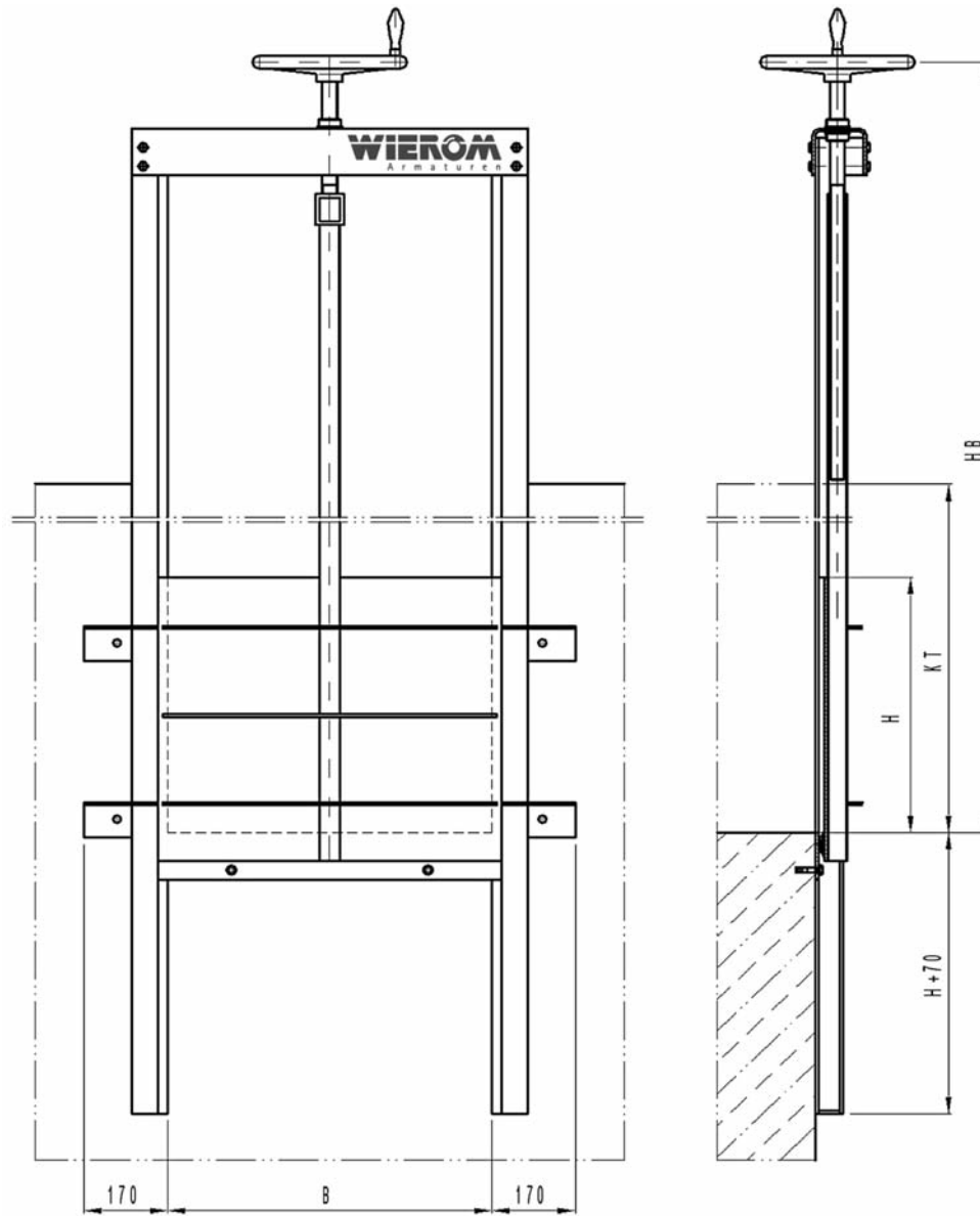
Detail: Side frame
