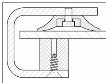
Detail: Side frame
