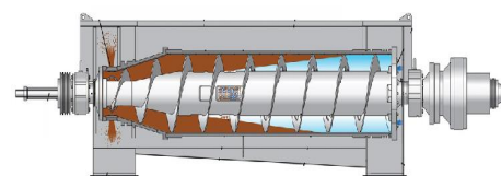
Example of 2-phases bowl configuration
