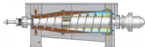
Example of 3-phases bowl configuration
