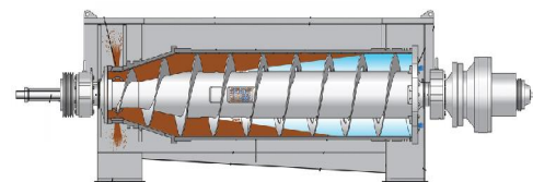
Example of 2-phases bowl configuration
