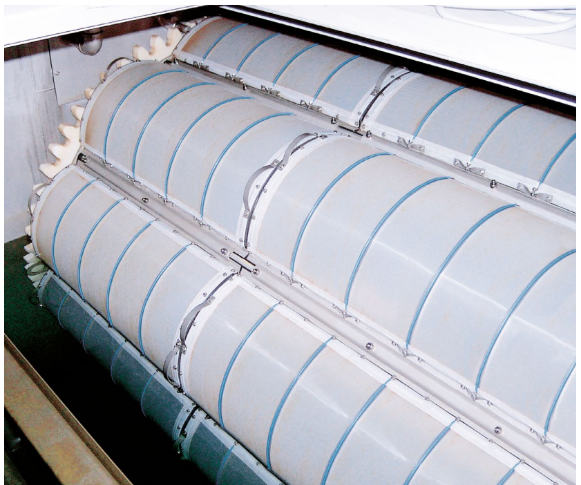
sieve baskets and sprocket, RSH-M
